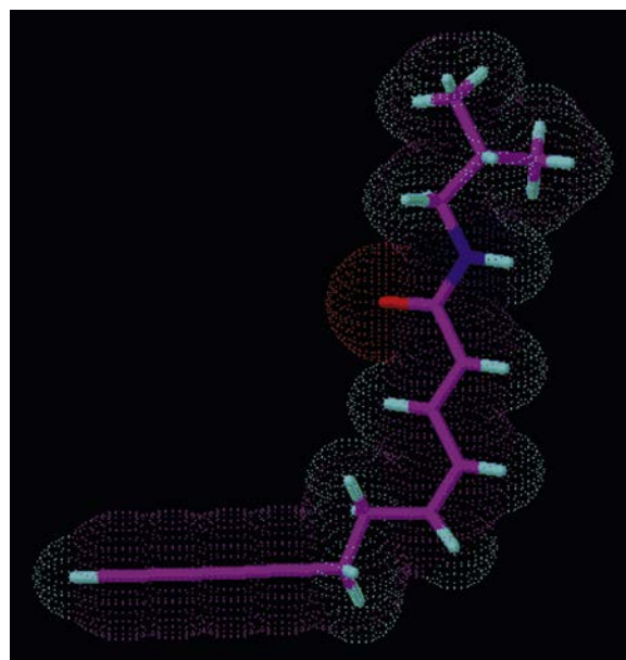
FIGURE A-4 Isobutylamide molecule. (Courtesy Lisa Ganora.)
