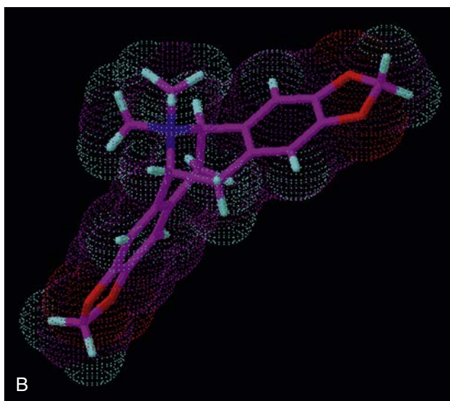
FIGURE A-8 A, California poppy ( Eschscholzia californica ). (Photo by Martin Wall.) B, Californidine molecule. (Courtesy Lisa Ganora.)
