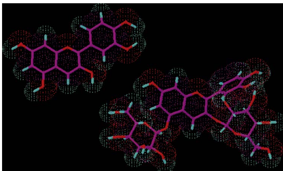
FIGURE A-6 Cyanidin molecule. (Courtesy Lisa Ganora.)
