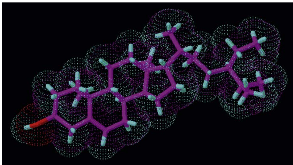
FIGURE A-7 Beta-sitosterol molecule. (Courtesy Lisa Ganora.)
